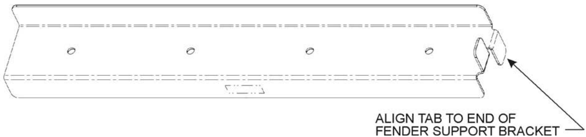
Figure 30. Drill Template (P/N 107406-1).
