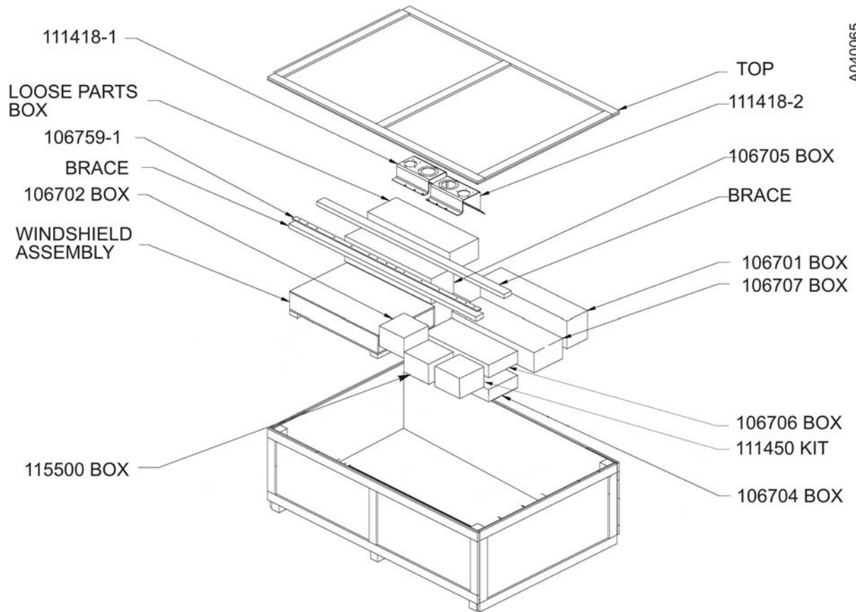
Figure 1-1. Crate No. 1 layout.
