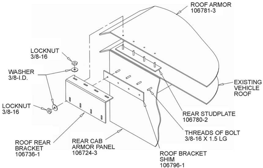
Figure 39. Roof Armor - rear driver's-side installation.
