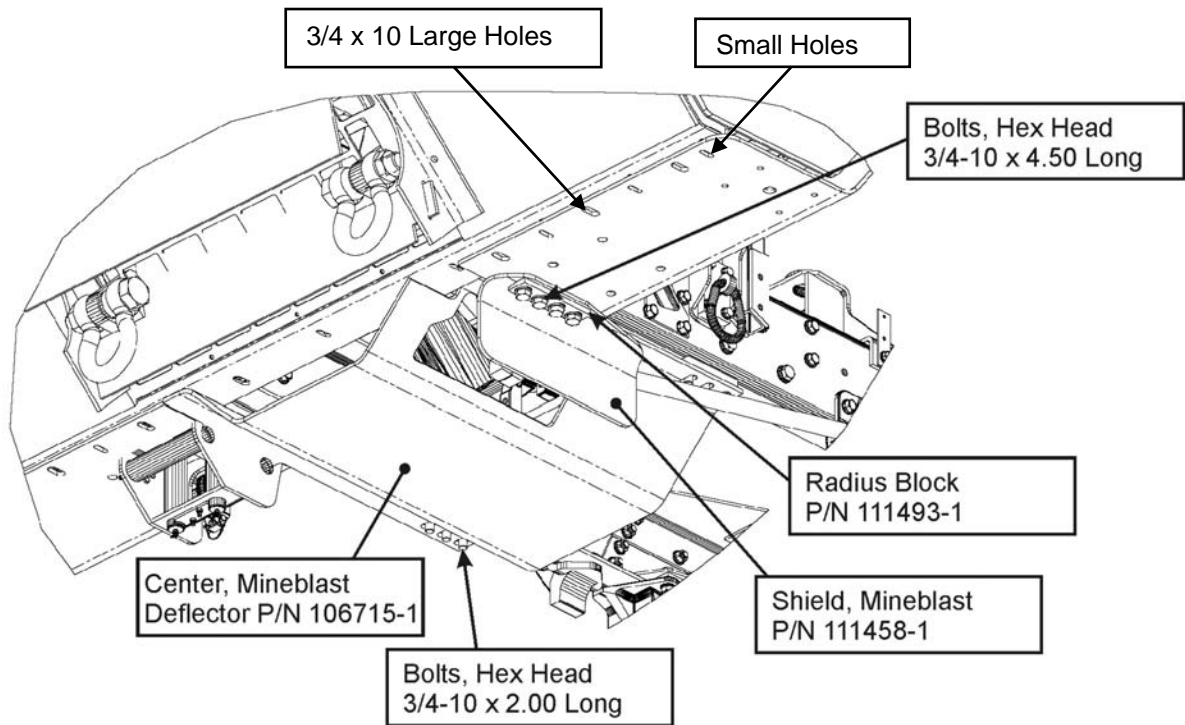
Figure 32. Secure the Center Blast Deflector to the Mounting Bracket.
