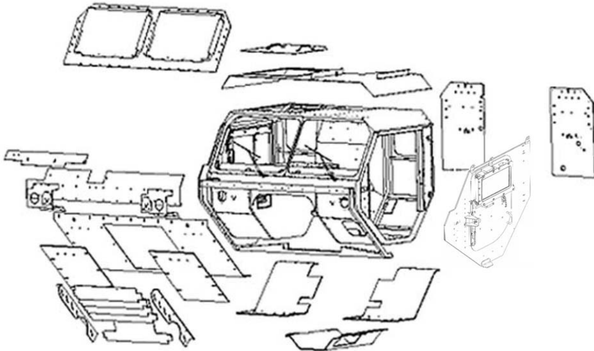
Figure 1. HEMTT Crew Protection Armor Kit component location.
