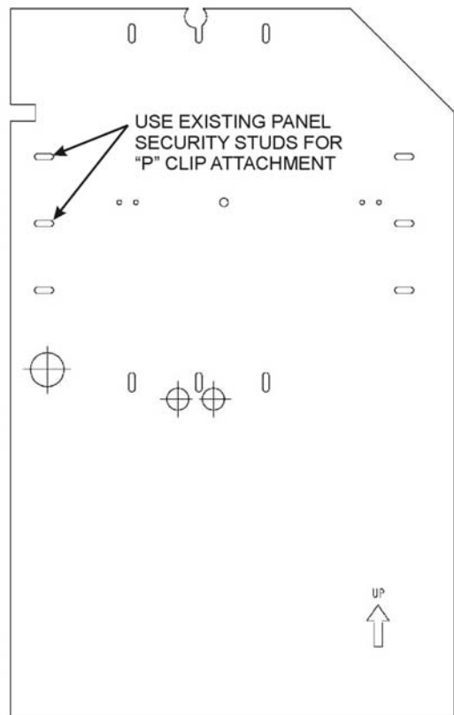
Figure 2.1. Right Rear Cab Armor Panel 106724-4 (Passenger Side).
