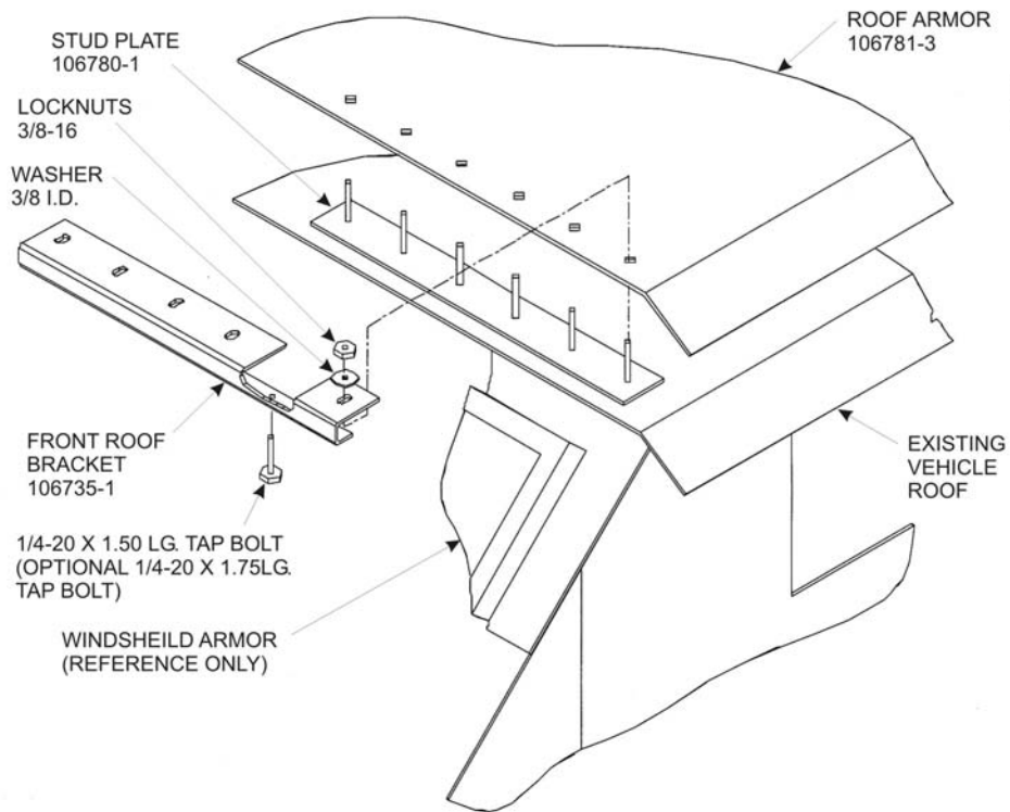
Figure 38. Roof Armor - front driver's-side installation.
